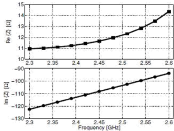
Fig. 2. Simulation results of the input impedance of the rectifier.
