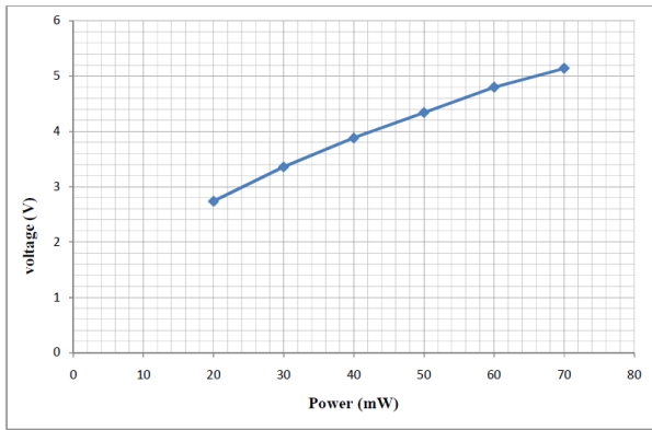
Fig. 5. Incident antenna power versus voltage.
