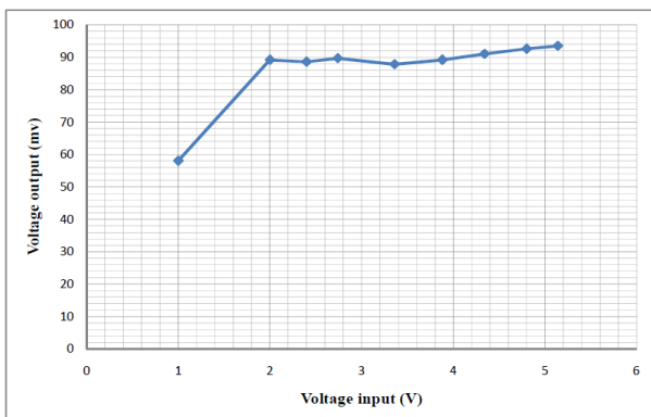
Fig. 6. Input and output voltage analysis.
