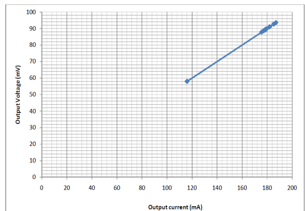
Fig. 7. Voltage-current characteristics.
