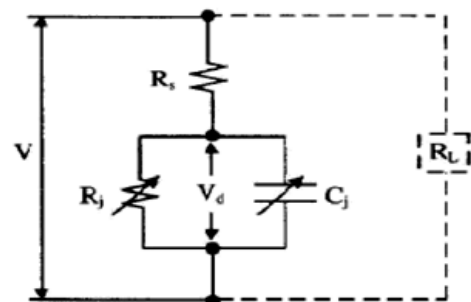
Fig. 3. Equivalent circuit model of the rectifying circuit.
